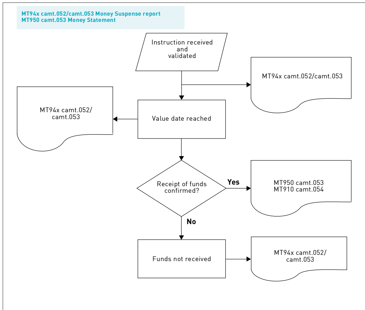
Figure 5.2 Life cycle of a Pre-advice of entry of funds
