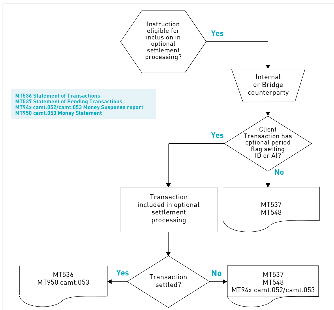
Figure 3.7 Flag setting requirements for optional settlement period processing
