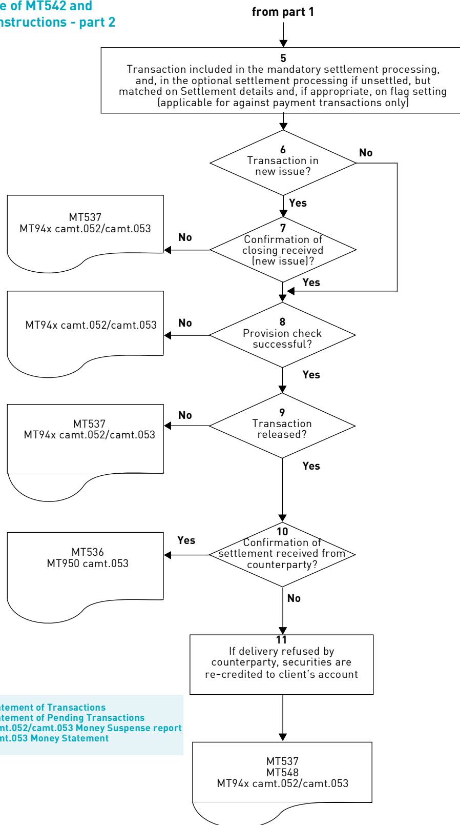
Figure 4.5 Life cycle of MT542 and MT543 instructions (Bridge deliveries) - part 2
