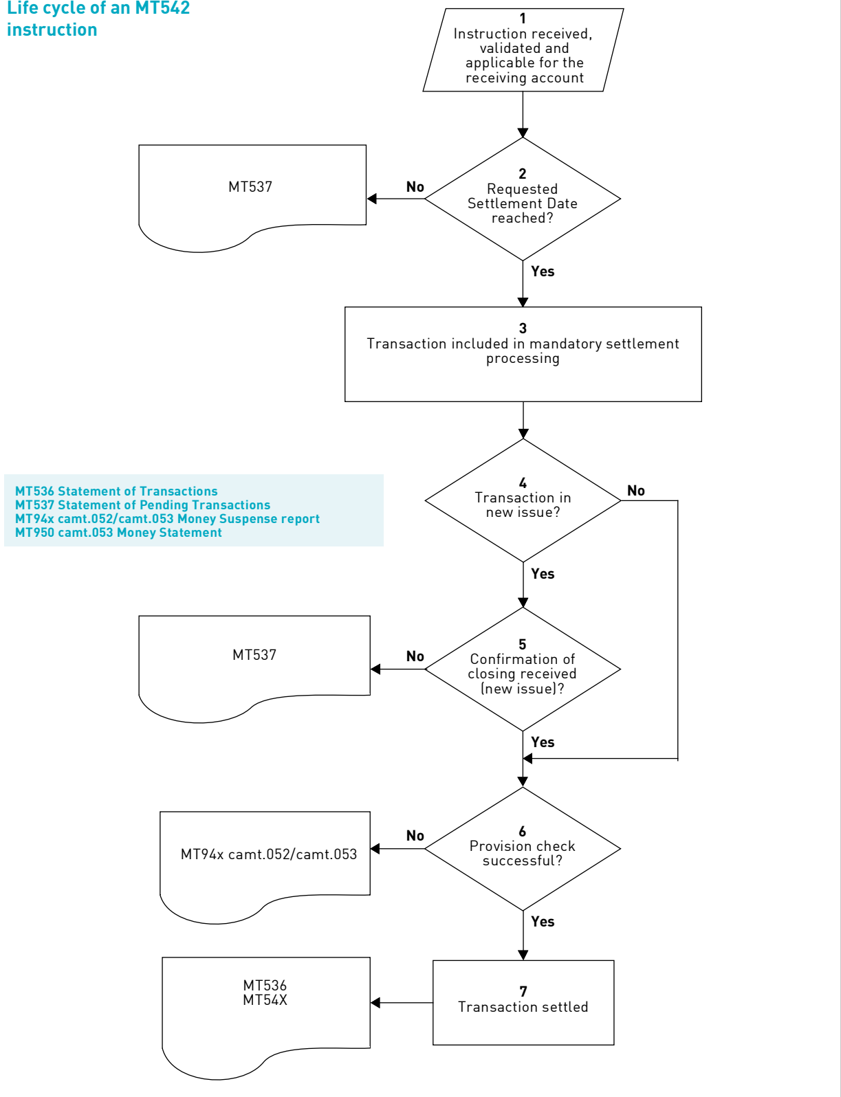
Figure 4.2 Life cycle of an MT542 instruction
